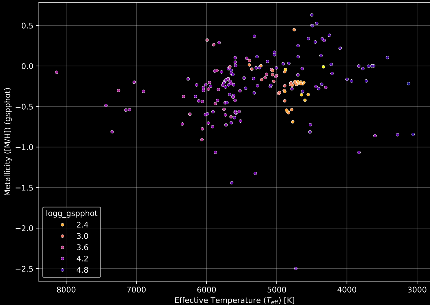
APOGEE DR17 Field: [176+37_MGA] Stellar Population Parameters (n= 187)
