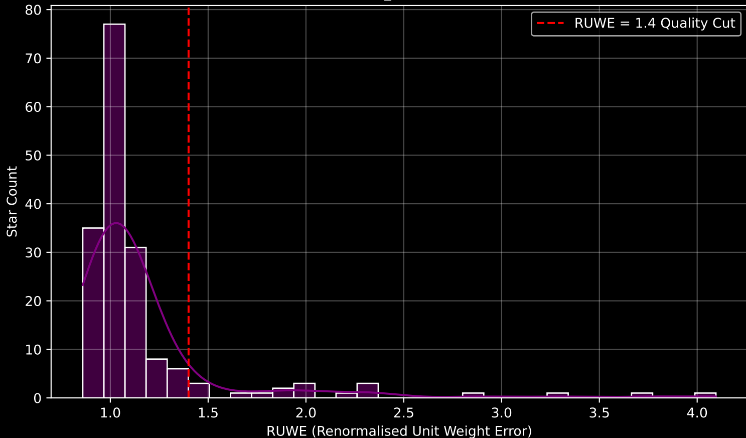
GAPOGEE DR17 Field [176+37_MGA] RUWE Distribution (n= 175)
