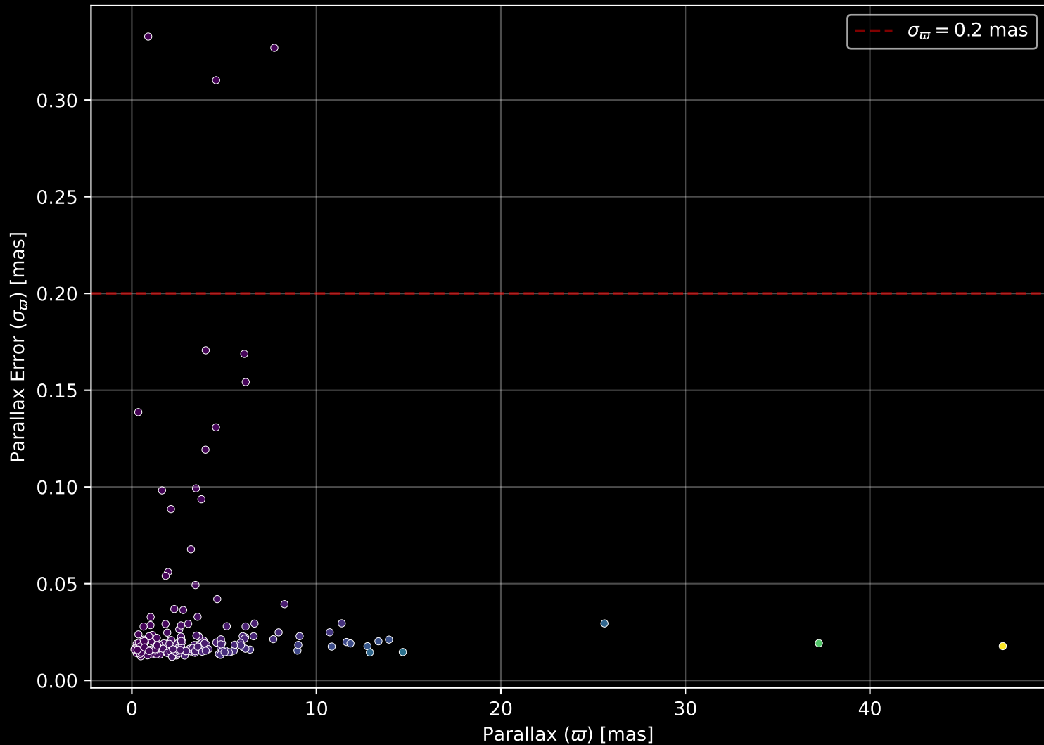
APOGEE DR17 Field: [176+37_MGA] Parallax Quality (n= 187)
