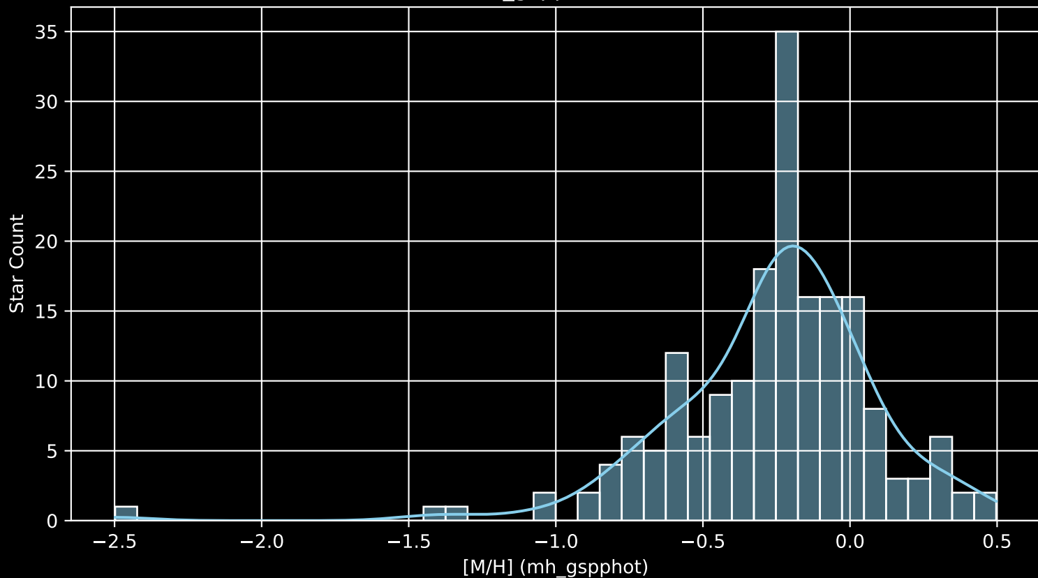
APOGEE DR17 Field: [176+37_MGA [M/H] (mh_gspphot) (n= 184)
