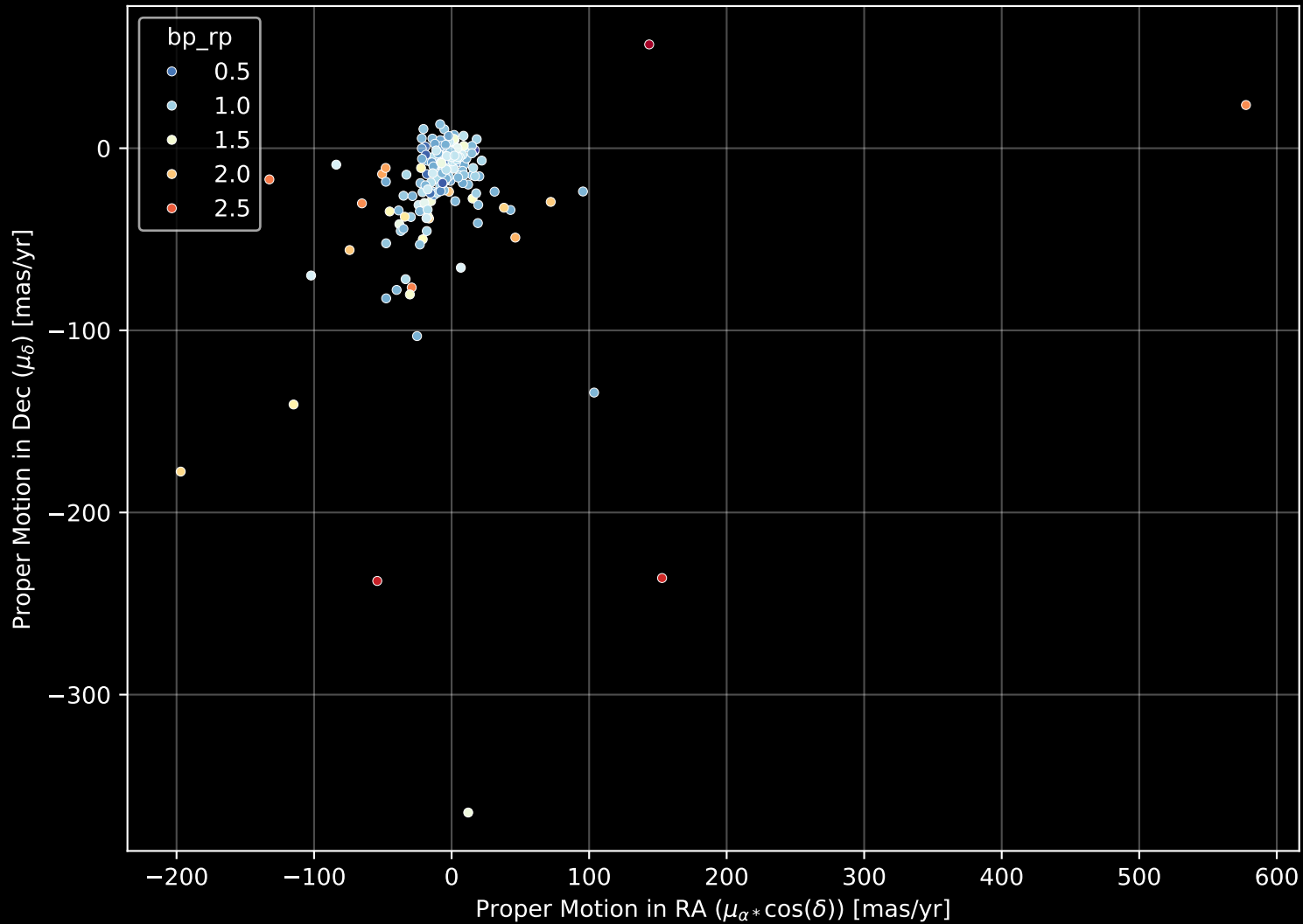
APOGEE DR17 Field: [176+37_MGA] Proper Motion Diagram (n= 187)
