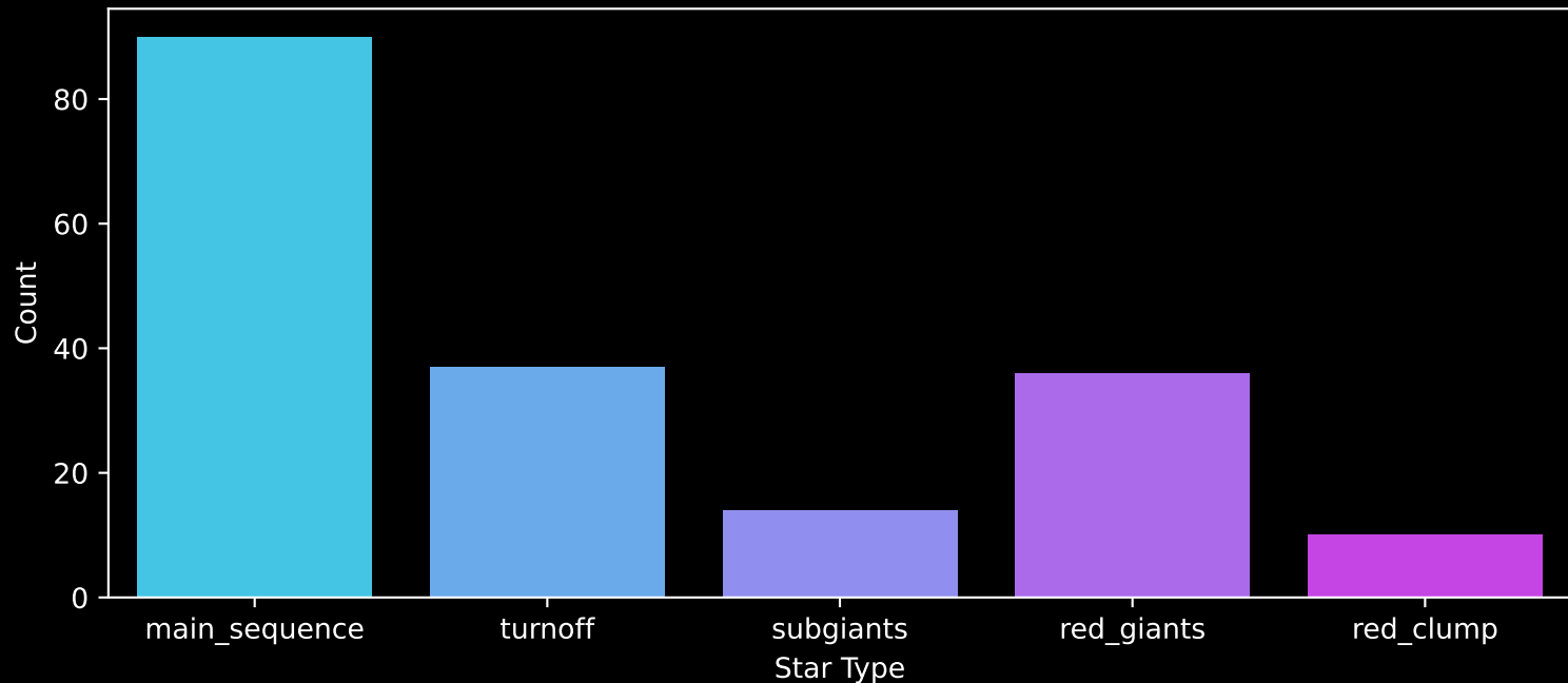
APOGEE DR17 Field: [176+37_MGA] Count plot of Star Type
